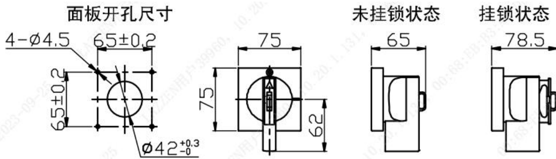
B-type handle size and mounting hole size
