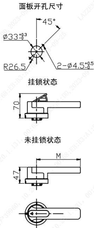
B-type handle size and mounting hole size
